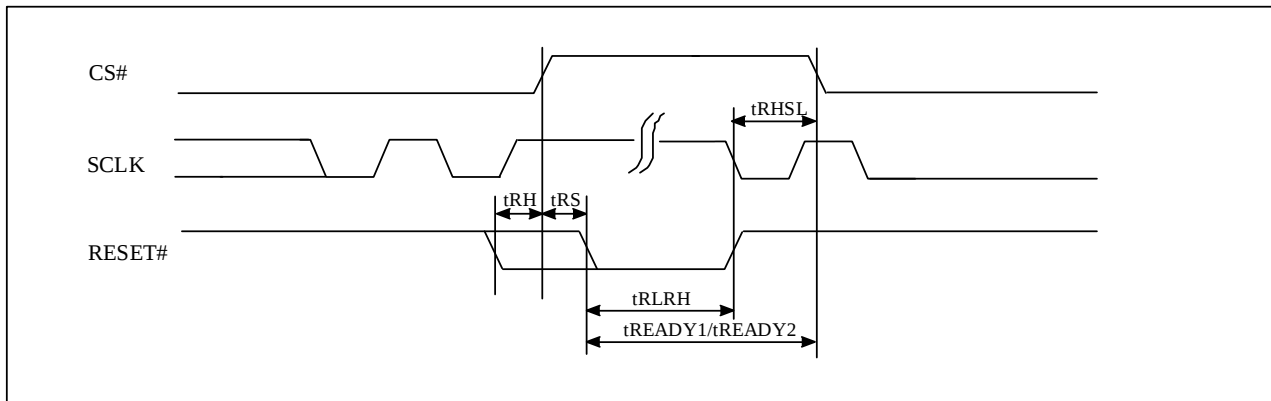
Figure 10-57 RESET Timing
