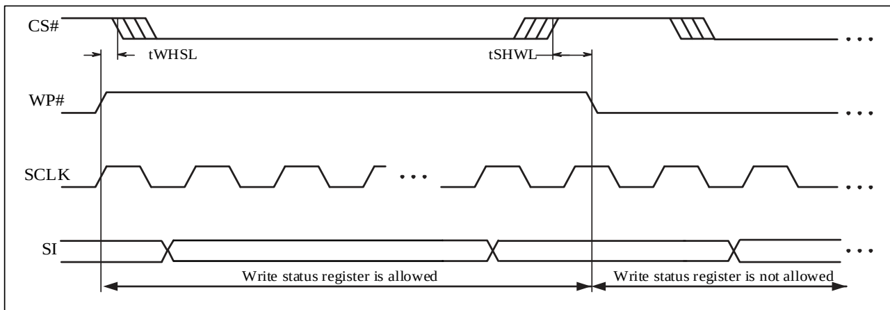
Figure 5-7 WP Timing
