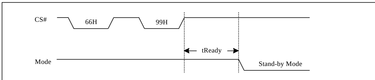
Figure 10-55a Reset Sequence
