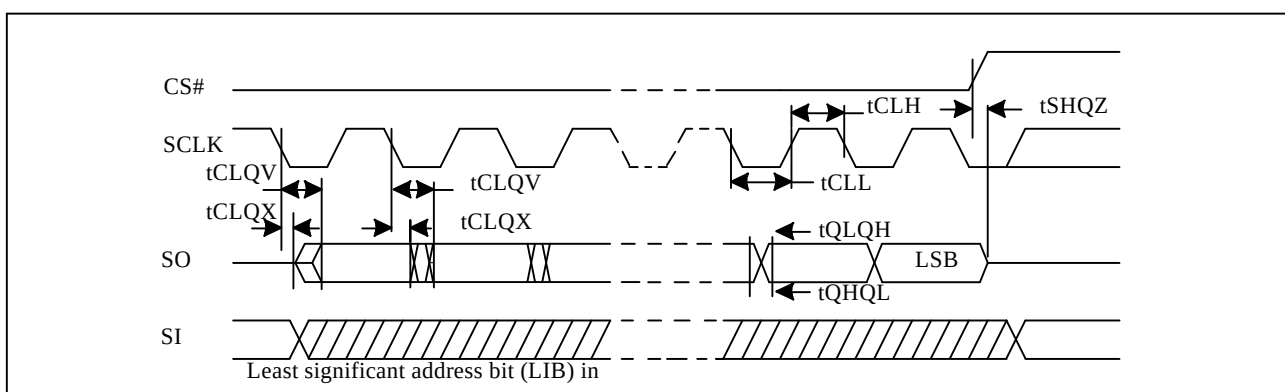
Figure 5-5 Output Timing
