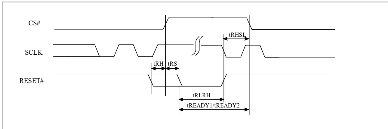
Figure 10-56 Reset Timing
