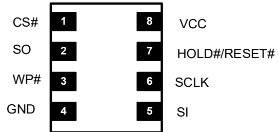
8-Pad USON (1.5x1.5mm/3x2mm)
