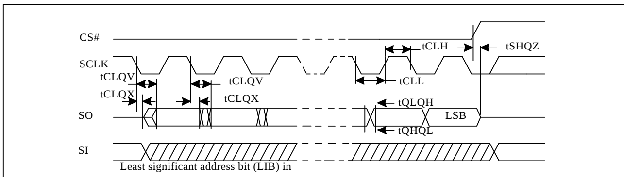
Figure 5-5 Output Timing
