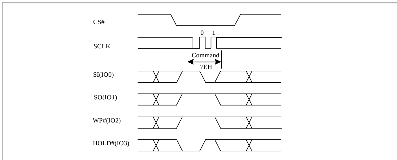
Figure 10-54a Global Block Lock(QPI)
