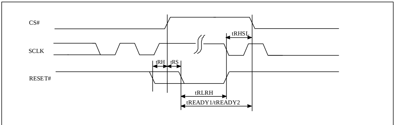
Figure 10-57 RESET Timing
