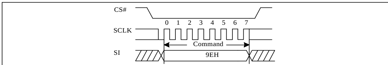
Figure 10-33 Buffer Clear Sequence (Command 9E)
