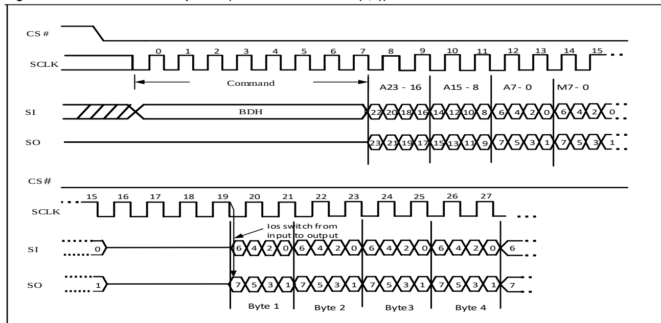
Figure 10-14 DTR 2IO Read Sequence (Command BD M5-4 ≠ (1,0))
