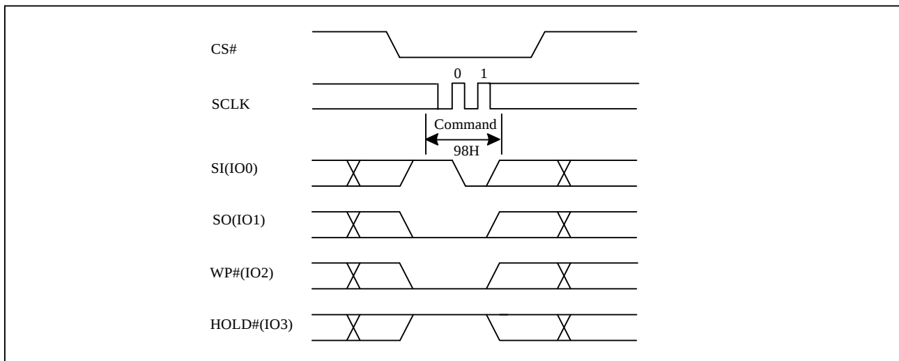
Figure 10-55a Global Block Unlock(QPI)
