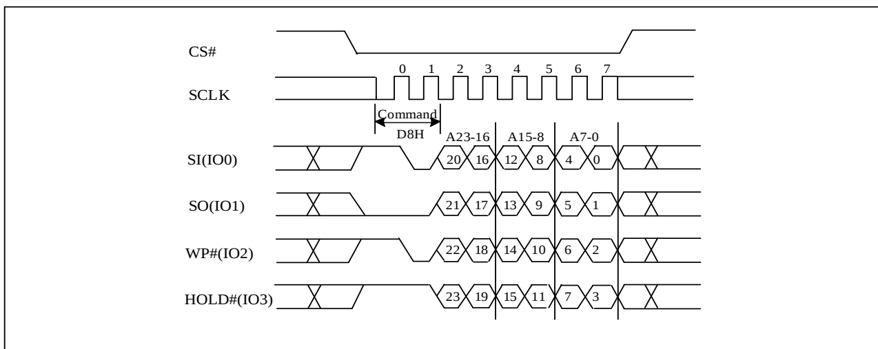
Figure 10-29a Block Erase (BE) sequence (QPI)
