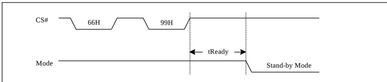
Figure 10-56a Reset Sequence
