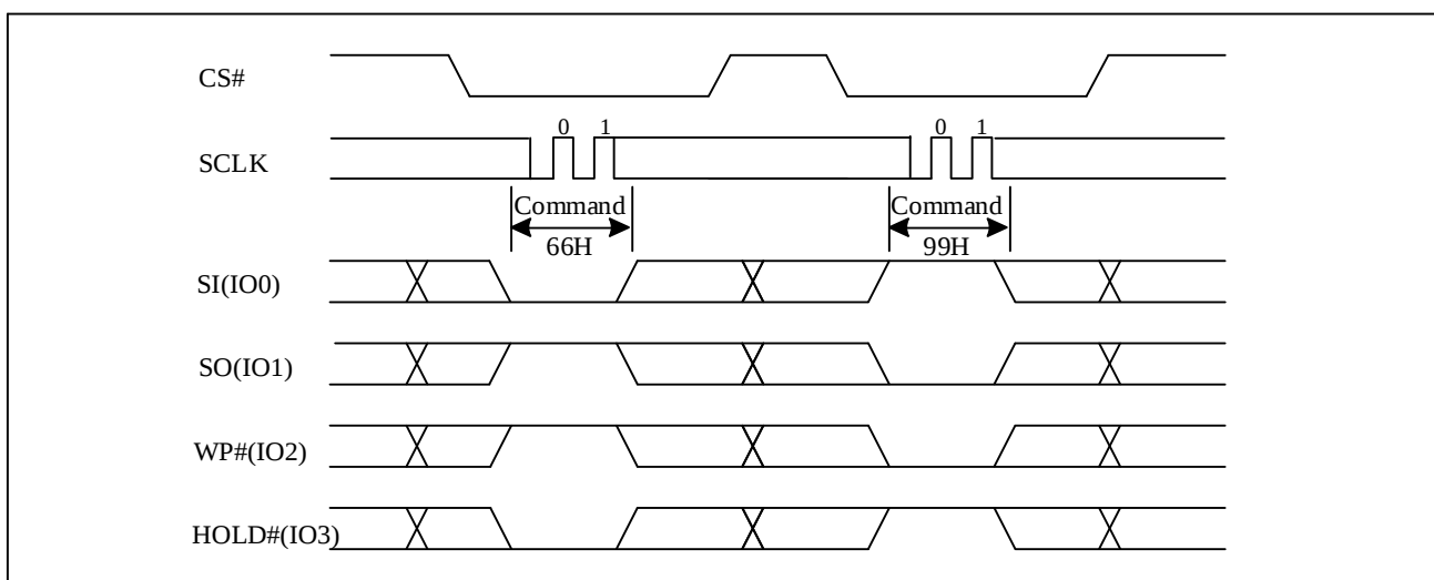
Figure 10-56b Reset Sequence(QPI)
