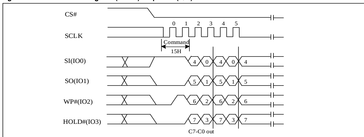
Figure 10-6a Read Status Register (RDCR) Sequence (QPI)
