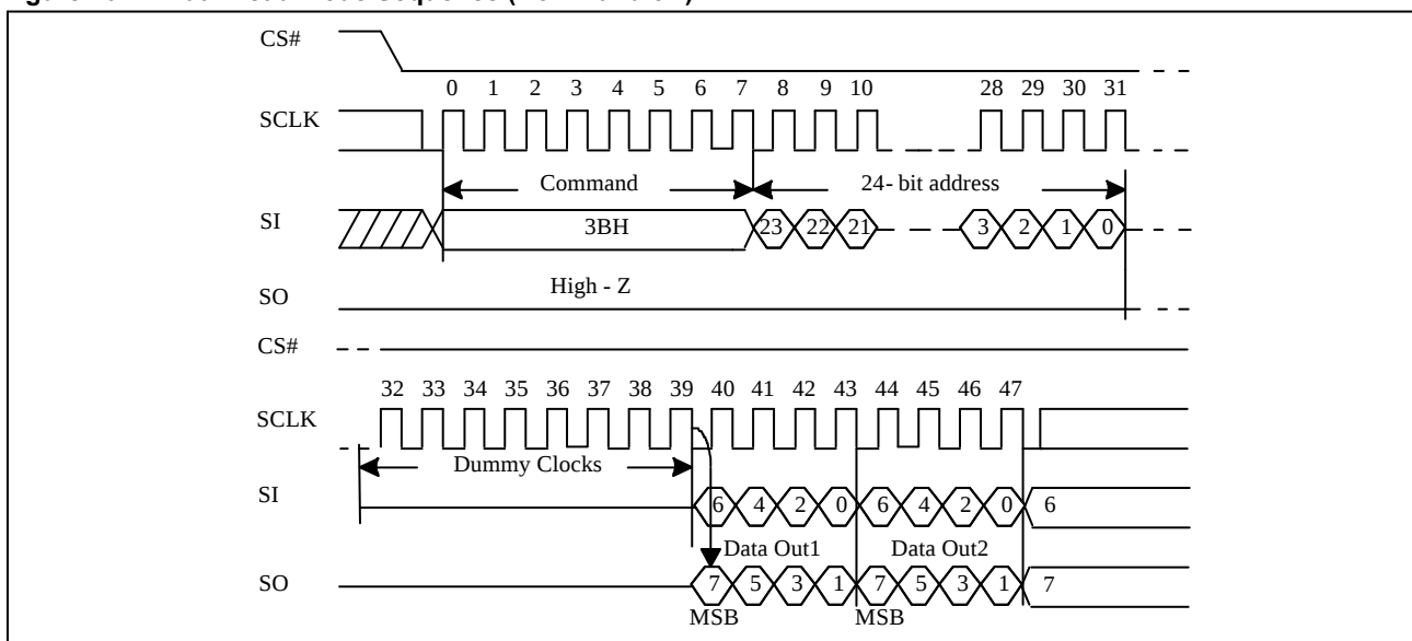
Figure 10-12 Dual Read Mode Sequence (Command 3B)
