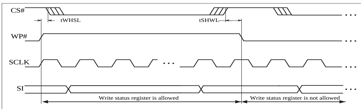
Figure 5-7 WP Timing
