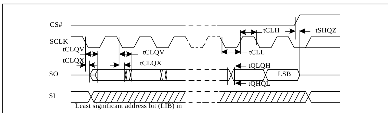
Figure 5-6 Hold Timing
