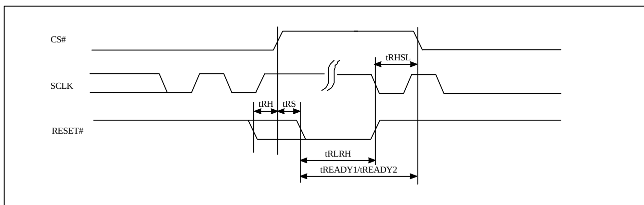
Figure 10-56 Reset Timing
