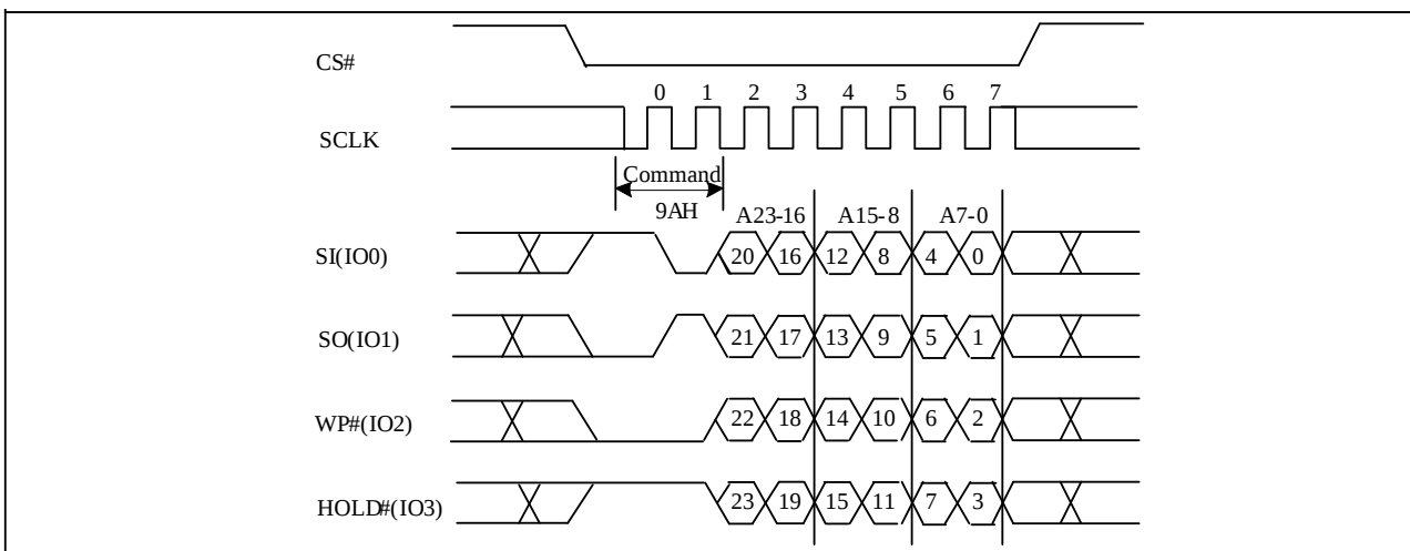
Figure 10-29b Buffer Load Sequence (QPI)
