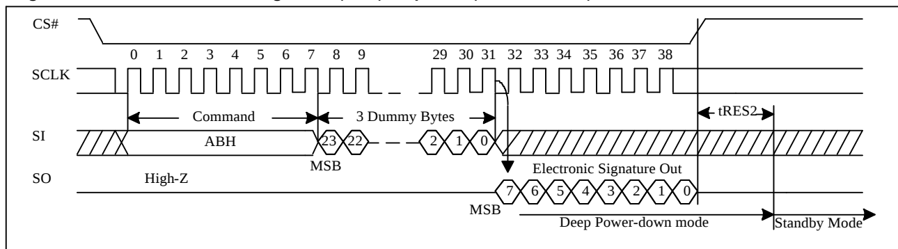
Figure 10-37a Read Electronic Signature (RES) Sequence (Command AB)
