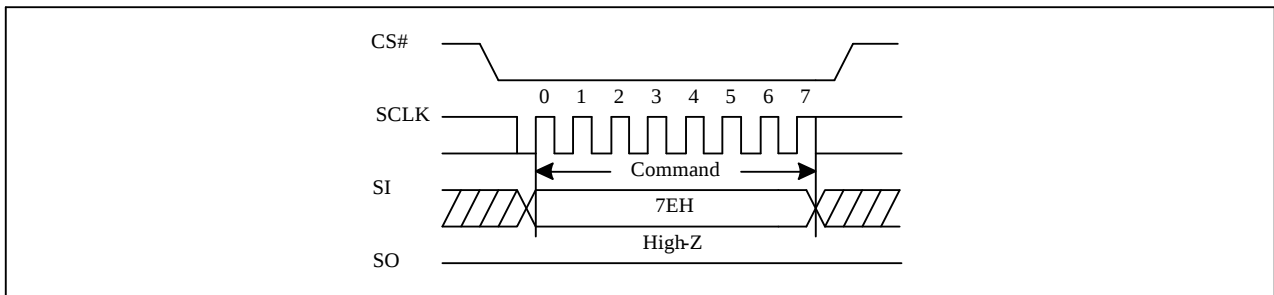
Figure 10-49b Global Block Lock(QPI)
