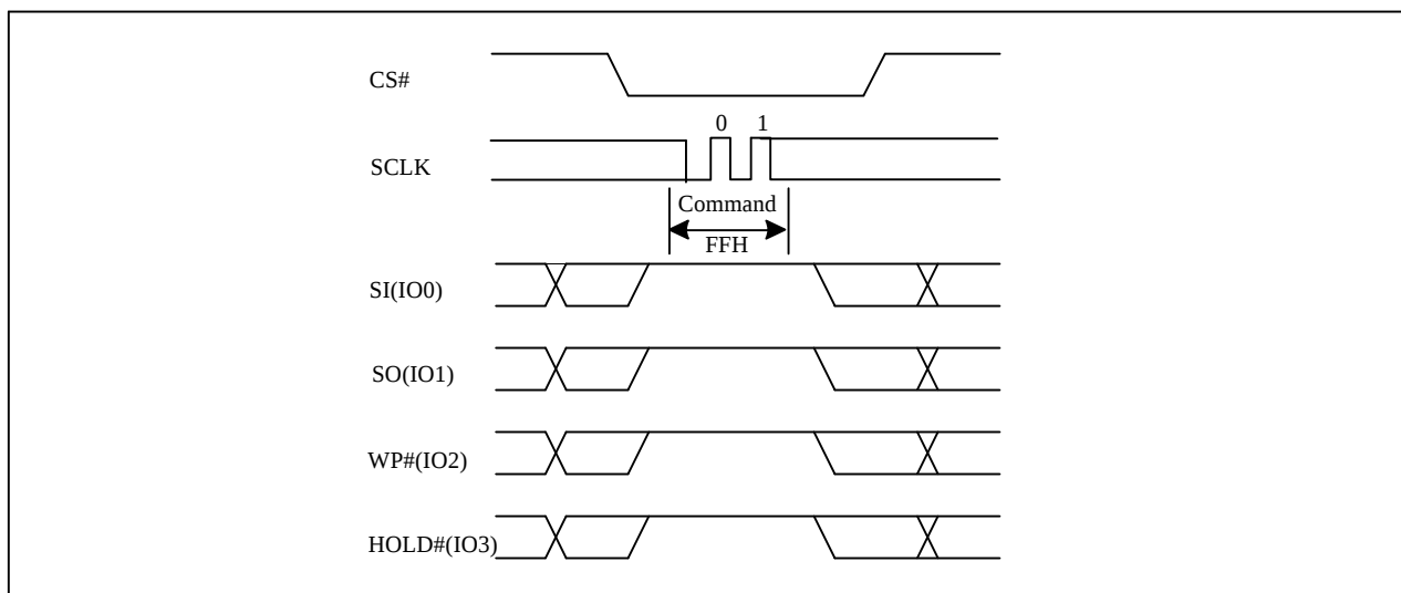
Figure 10-20 Disable QPI Sequence (QPI)
