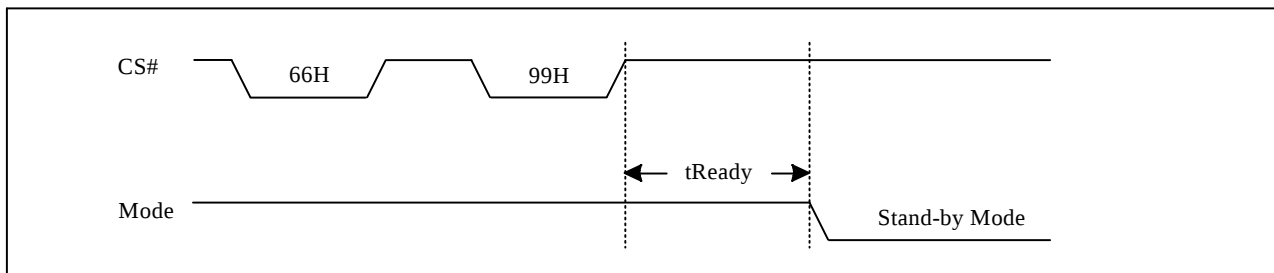
Figure 10-51b Reset Sequence
