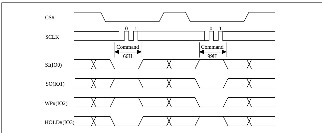
Figure 10-51c Reset Sequence(QPI)
