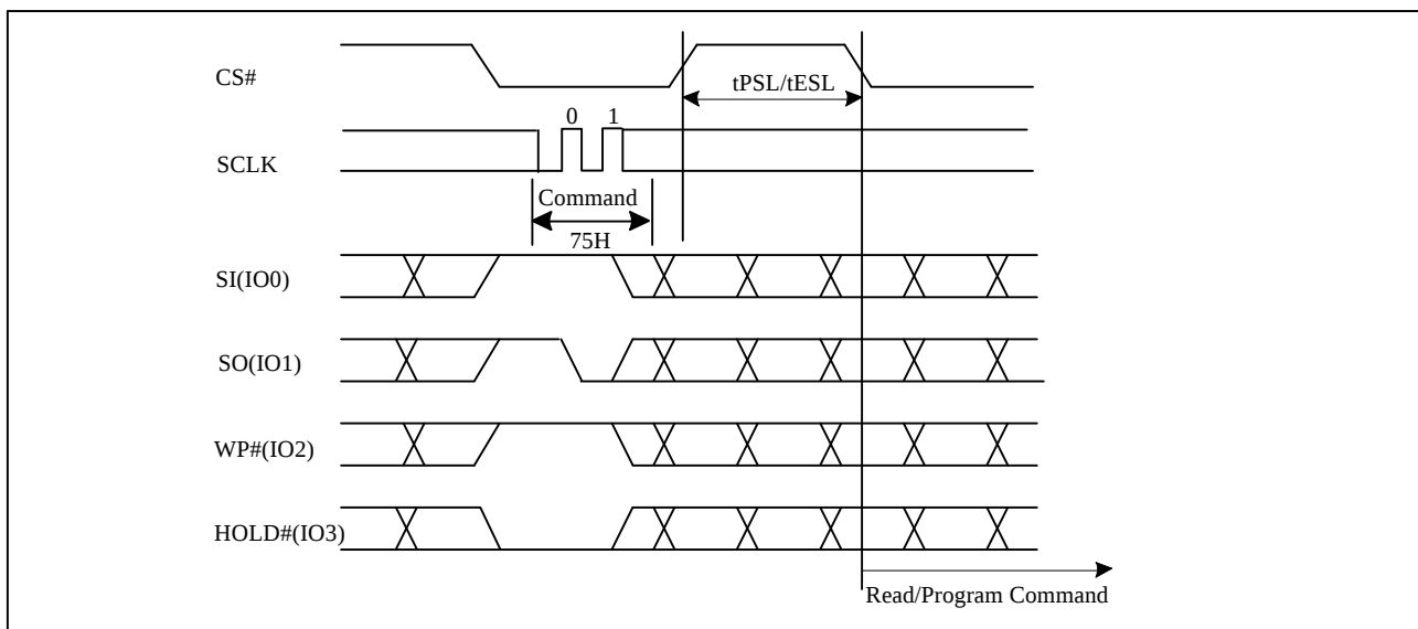
Figure 10-43b Suspend to Read/Program Latency(QPI)
