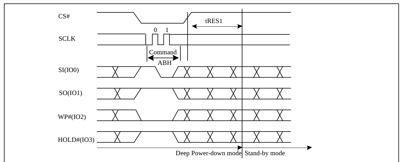
Figure 10-37d Release from Deep Power-down (RDP) Sequence (QPI)
