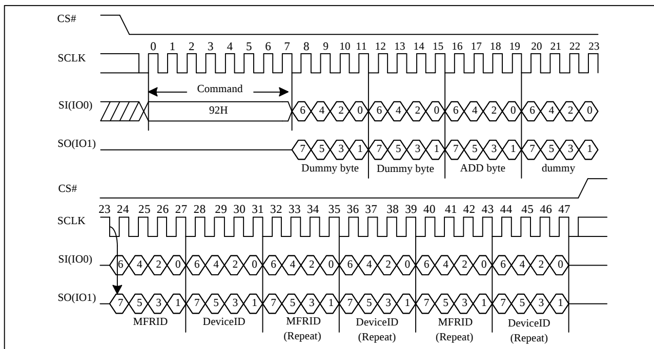
Figure 10-39 DUAL I/O Read Electronic Manufacturer & Device ID (DREMS) Sequence (Command 91)
