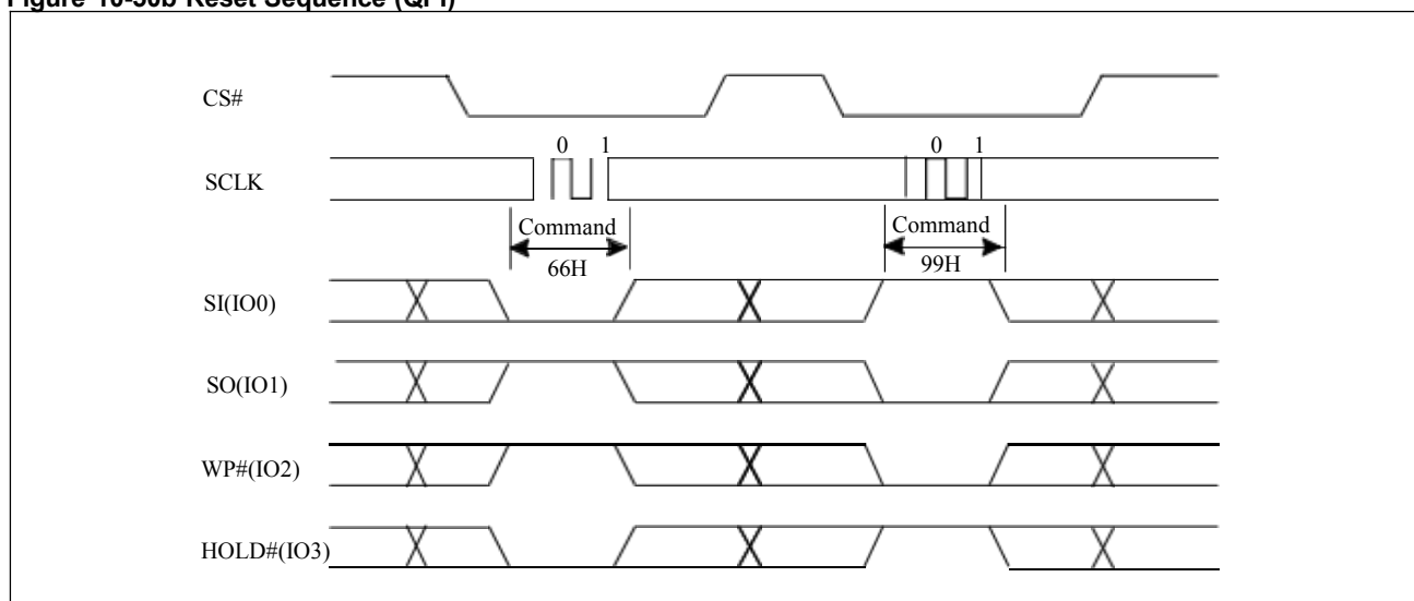
Figure 10-50b Reset Sequence (QPI)
