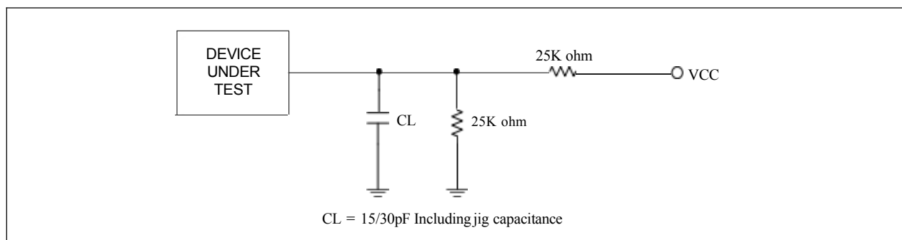
Figure 5-3 Output Loading
