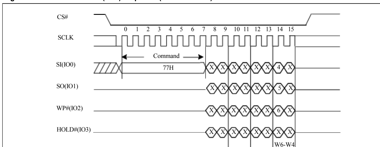
Figure 10-17 Set Burst Read (SBL) Sequence (Command 77h)
