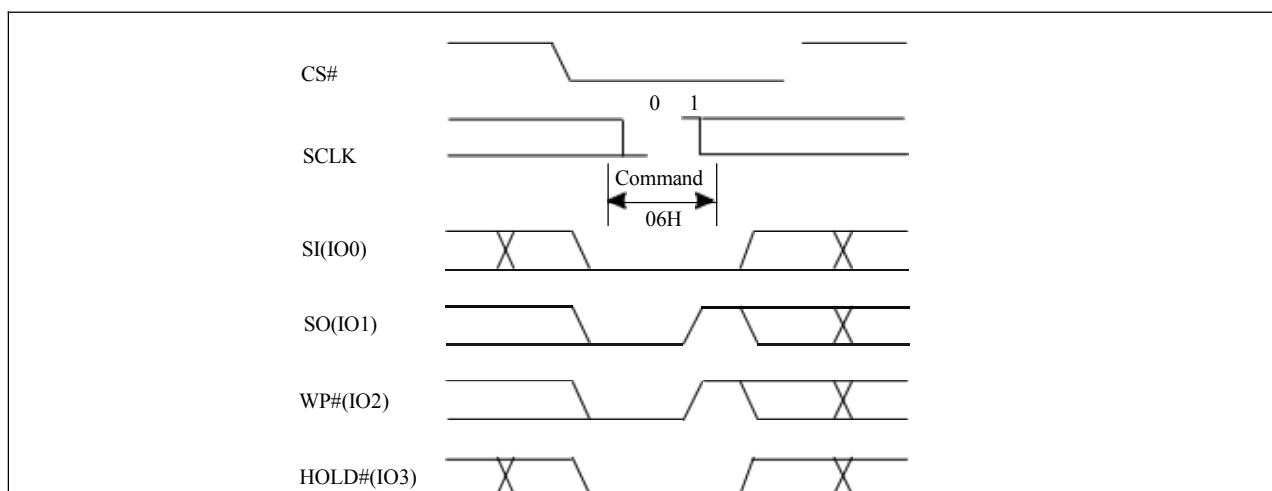
Figure 10-2a Write Enable (WREN) Sequence (QPI)
