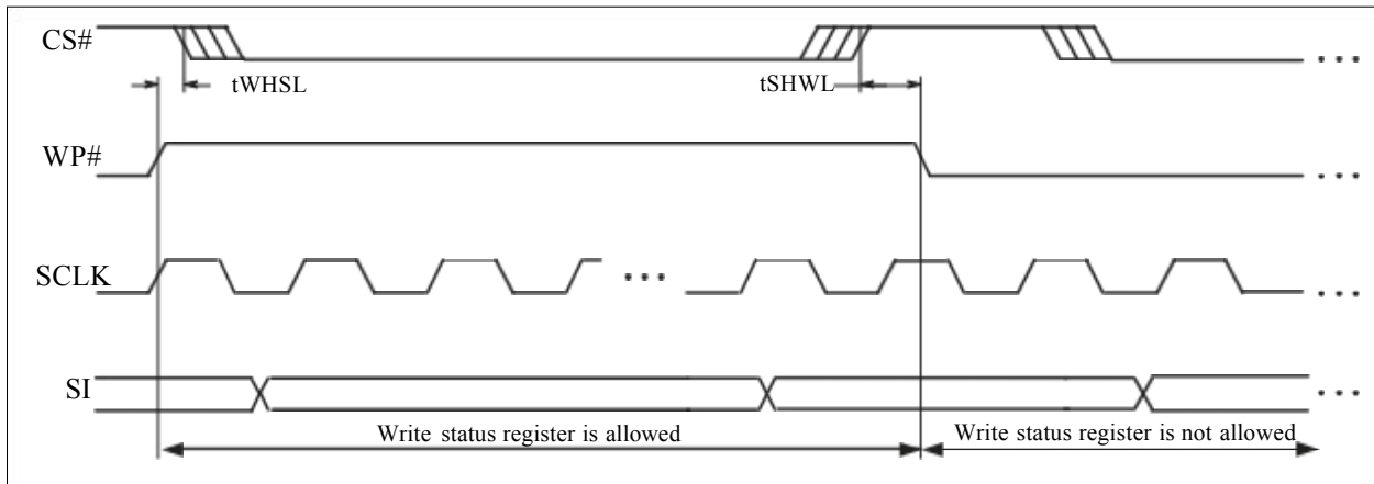
Figure 5-7 WP Timing
