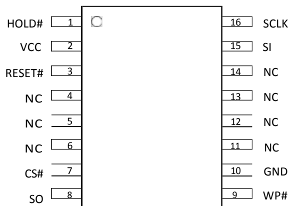
16-PinSOP (300mil)
