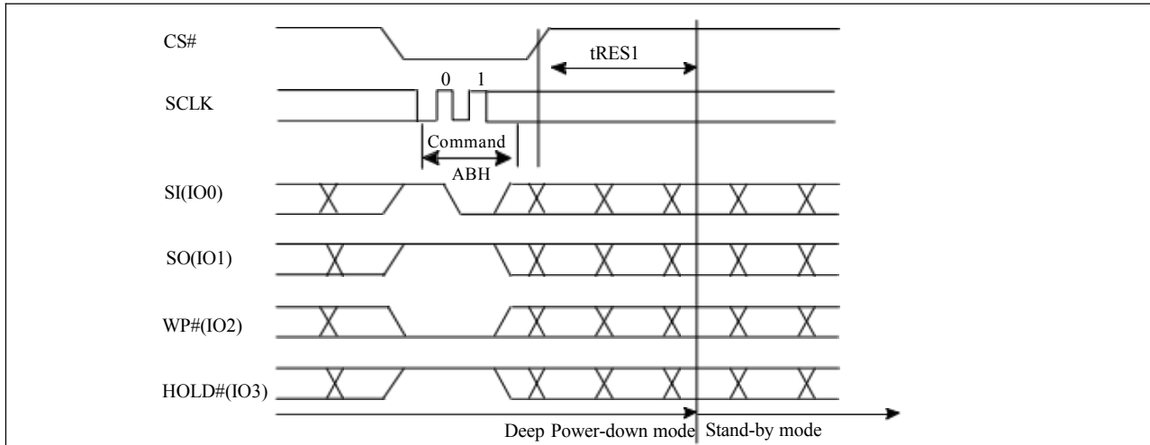
Figure 10-36c Release from Deep Power-down (RDP) Sequence (QPI)
