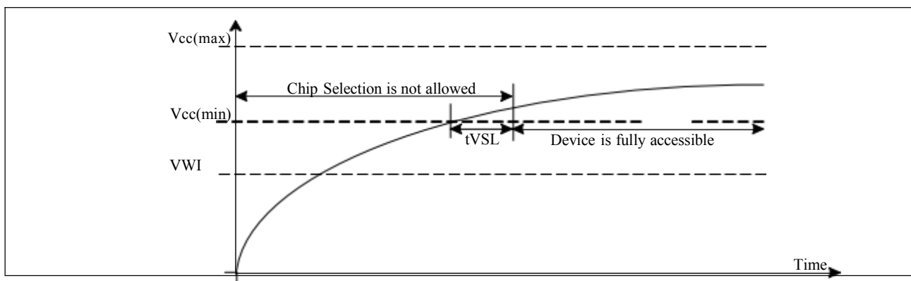
Figure 5-9 Power-Up Timing
