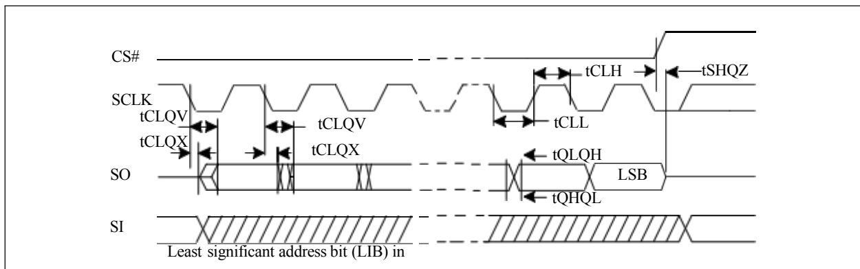
Figure 5-6 Hold Timing
