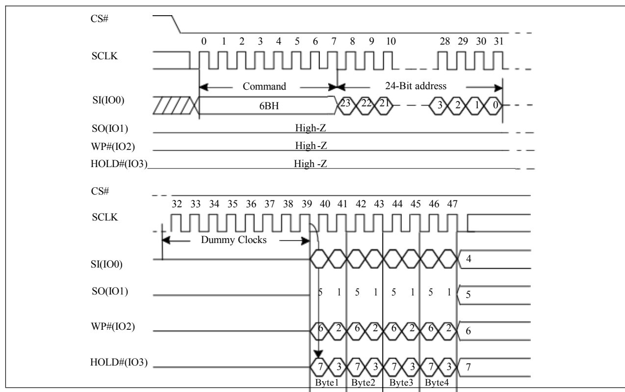
Figure 10-15 Quad Read Sequence (Command 6Bh)
