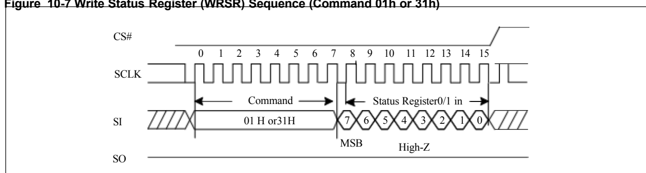
Figure 10-7 Write Status Register (WRSR) Sequence (Command 01h or 31h)
