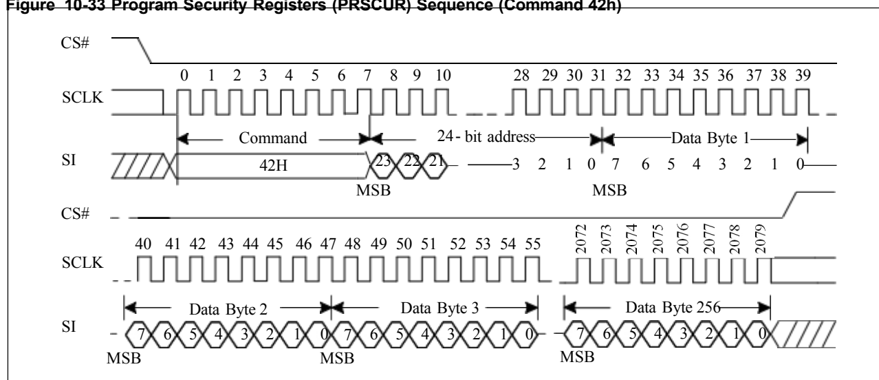
Figure 10-33 Program Security Registers (PRSCUR) Sequence (Command 42h)
