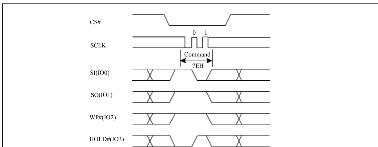
Figure 10-48a Global Block Lock (QPI)
