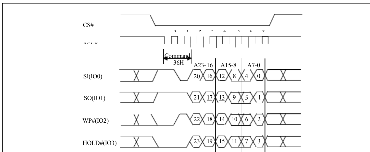
Figure 10-45a Individual Block Lock (QPI)
