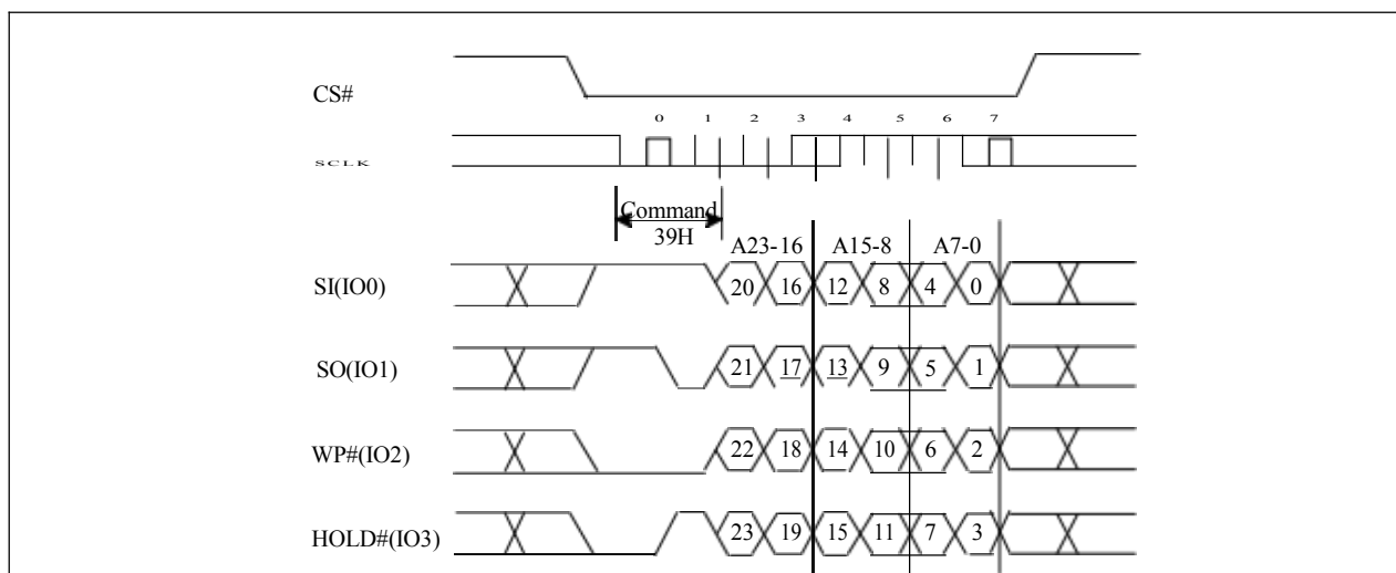
Figure 10-46a Individual Block Unlock (QPI)
