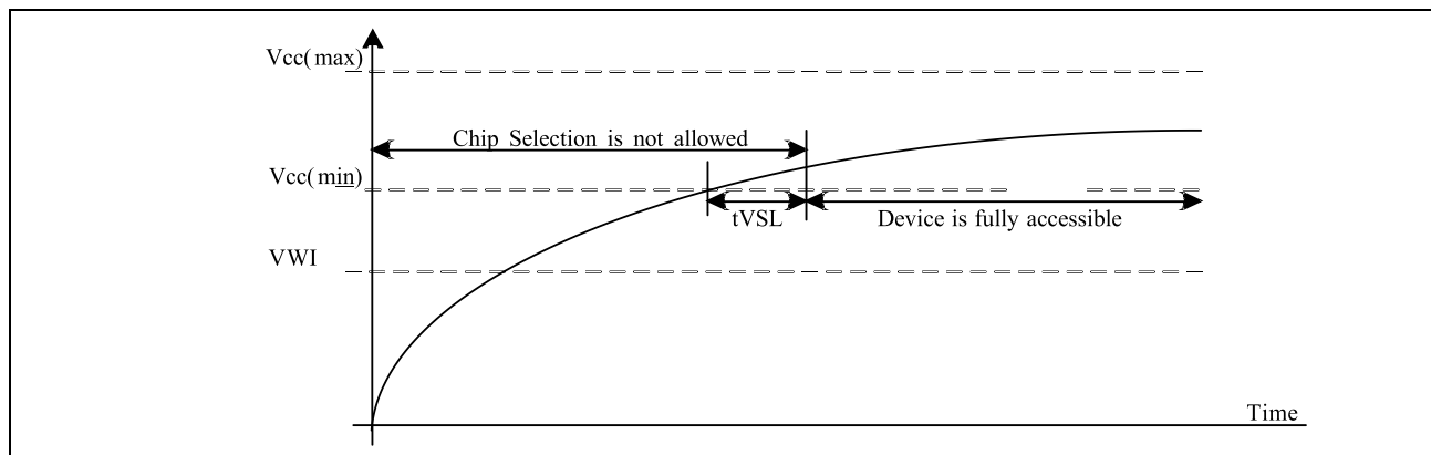
Figure9-9 Power-up Timing
