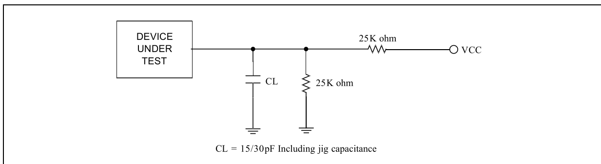
Figure 9-3 Output Loading
