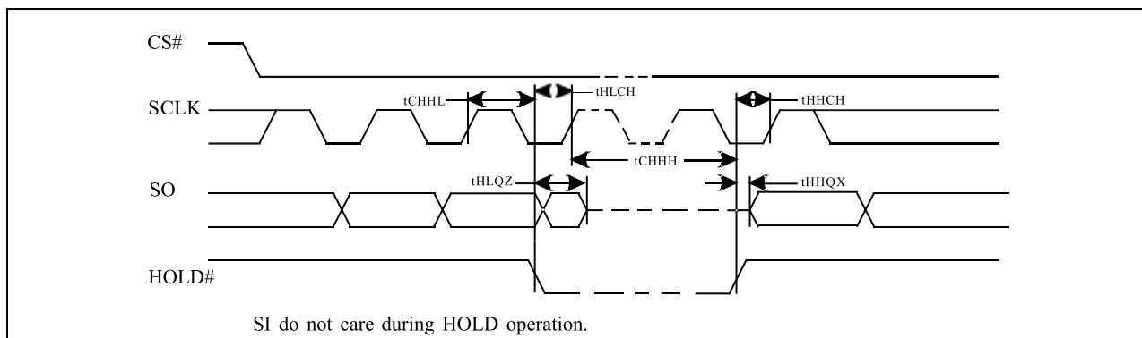
Figure 9-6 Hold Timing
