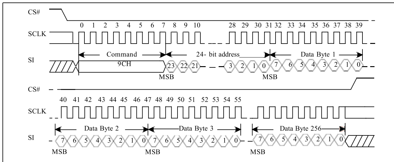
Figure 10-38 Buffer Write Sequence (Command 9Ch)
