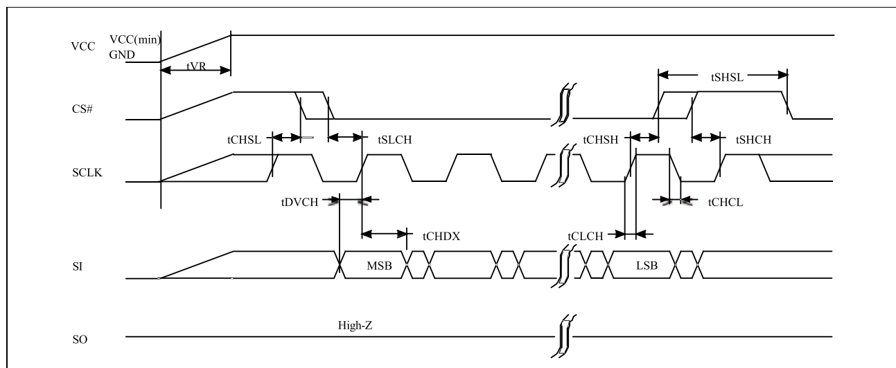
Figure9-9 Power-up Timing
