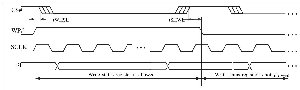
Figure 9-7 WP Timing
