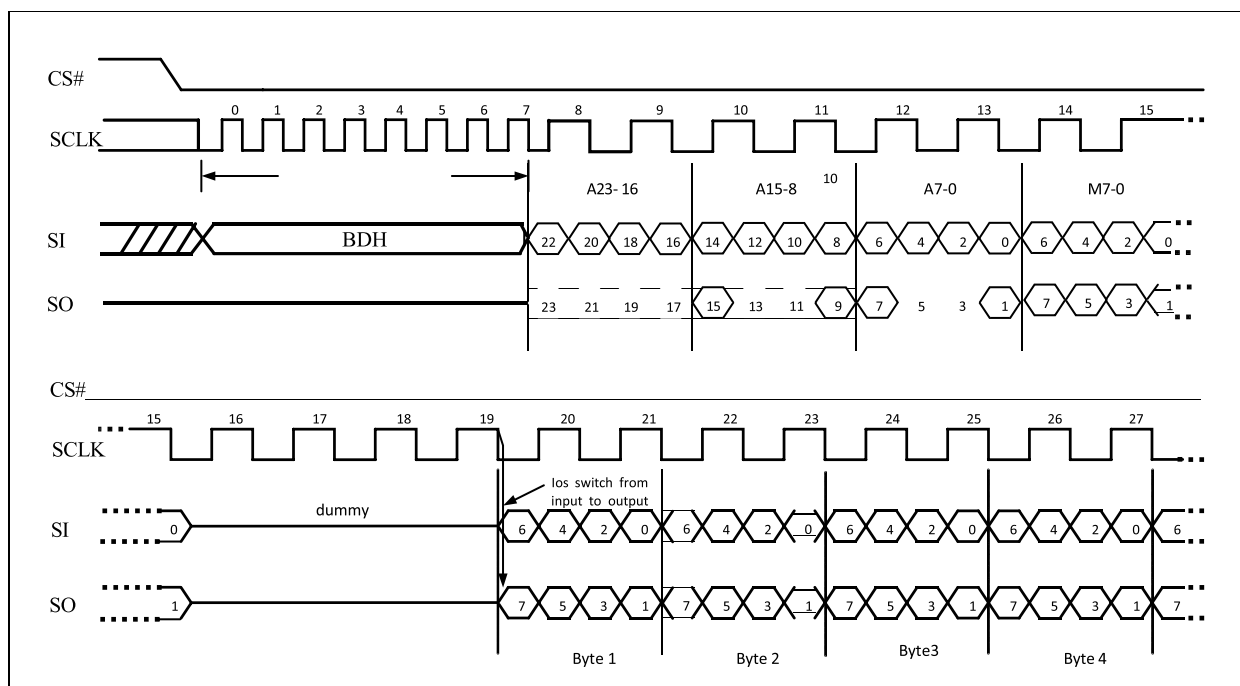
Figure 10-16 DTR 2IO Read Sequence (Command BDH M5-4 ≠ (1,0))
