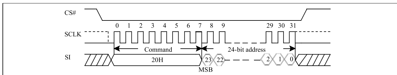
Figure 10-29 Sector Erase (SE) Sequence (Command 20h)
