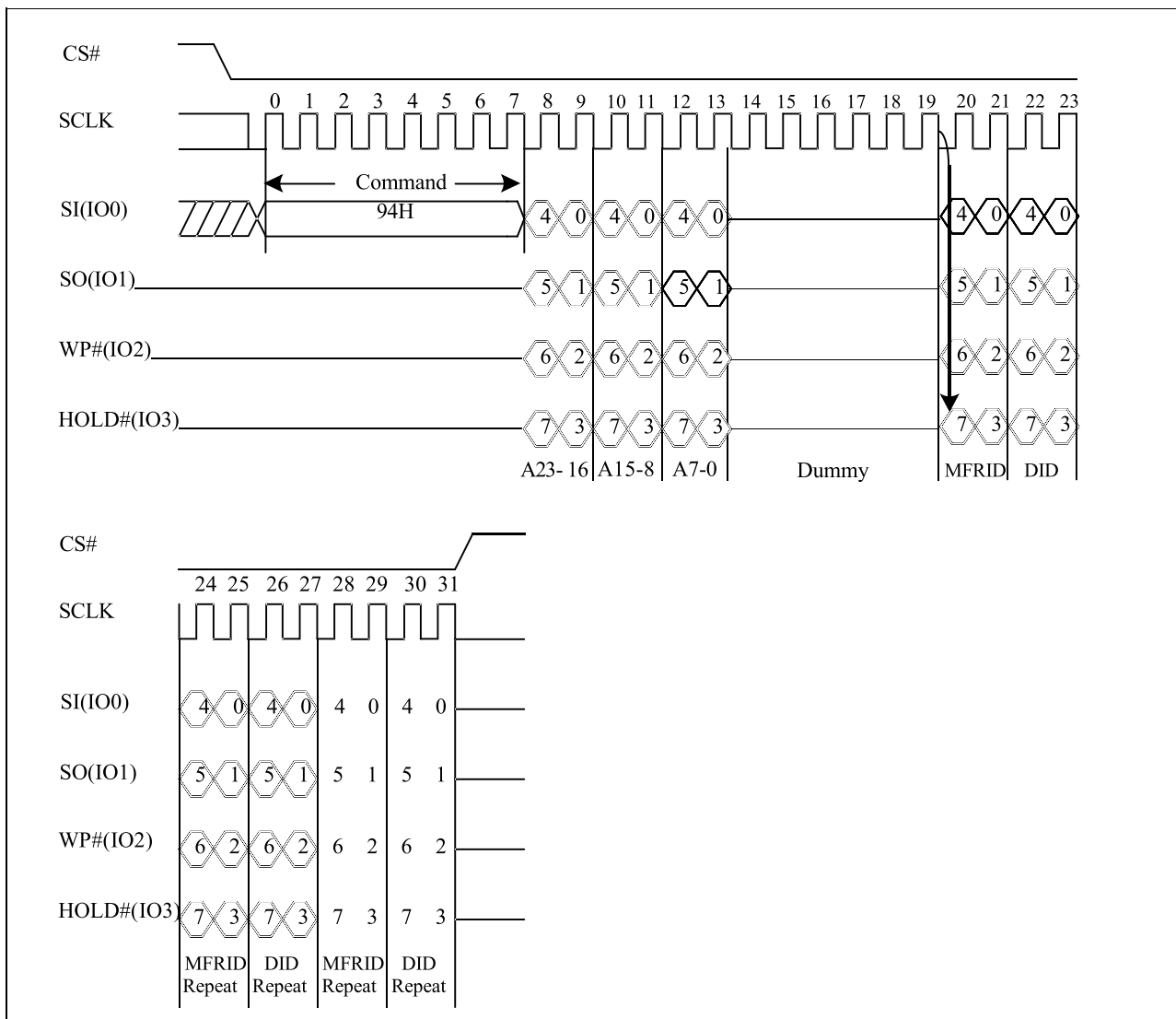
Figure 10-47 QUAD I/O Read Electronic Manufacturer &amp; Device ID (QREMS) Sequence (Command 94h)
