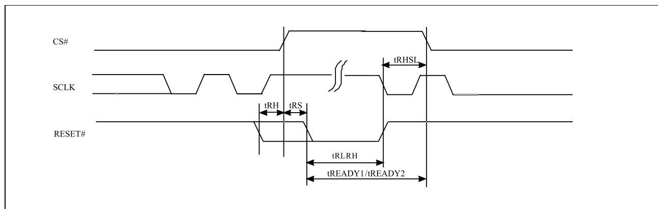
Figure 10-59 RESET Timing
