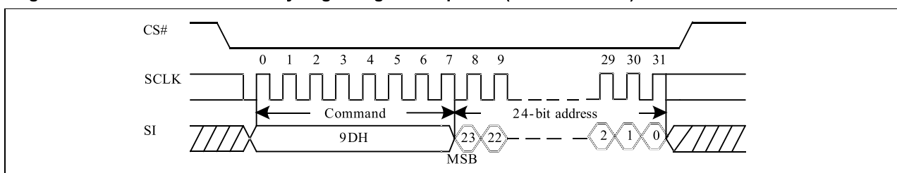
Figure 10-39 Buffer to Main Memory Page Program Sequence (Command 9Dh)
