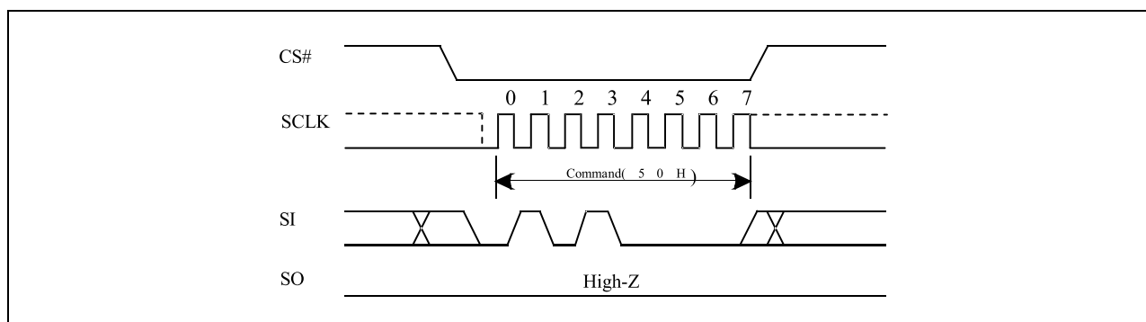
Figure 10-4 Write Enable for Volatile Status Register Sequence (Command 50h)
