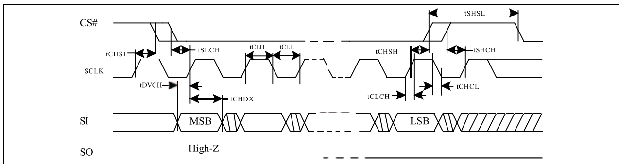
Figure 9-4b Serial Input Timing in DTR Mode
