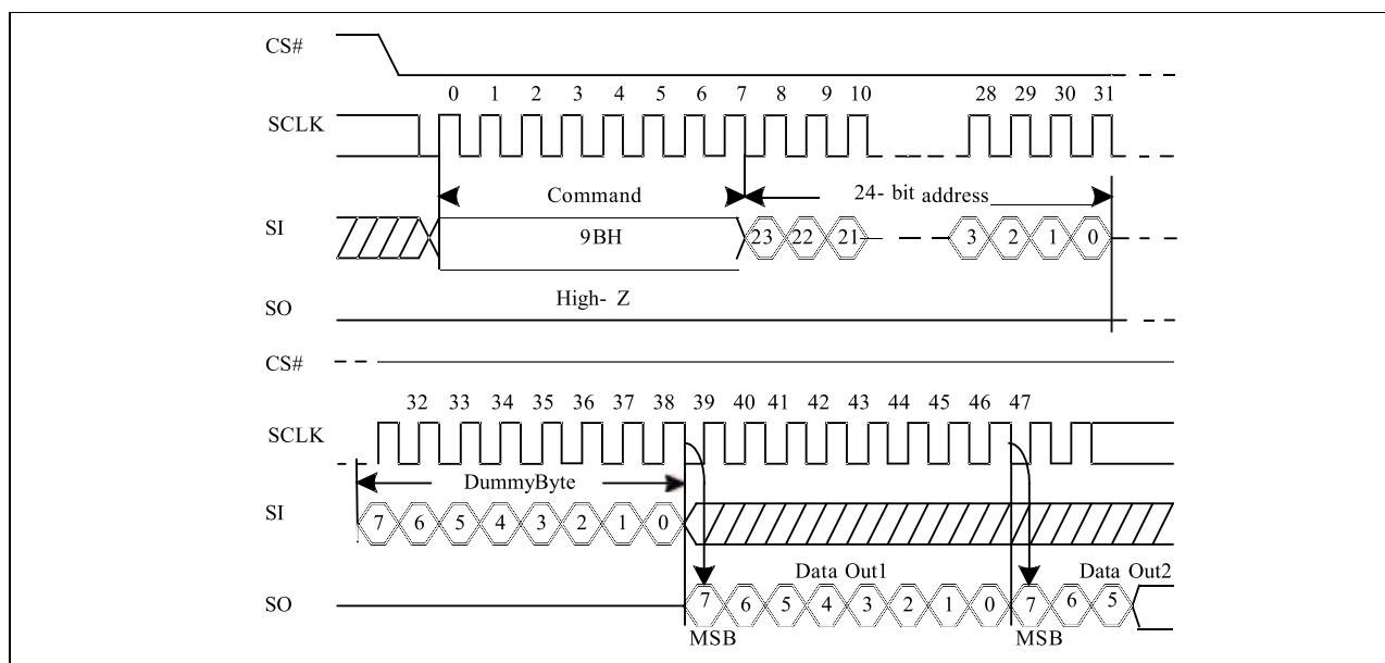
Figure 10-37 Buffer Read Sequence (Command 9Bh)
