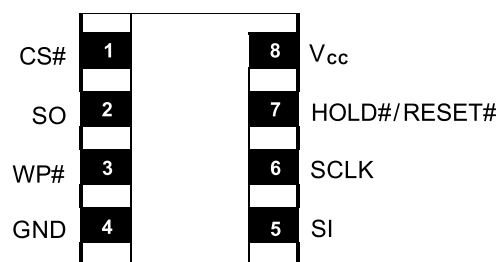
8-Land USON (4x4mm/6x5mm)
