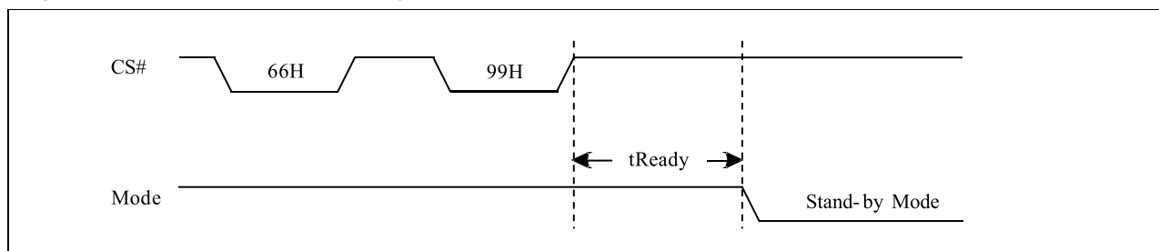
Figure 10-58a Reset Sequence
