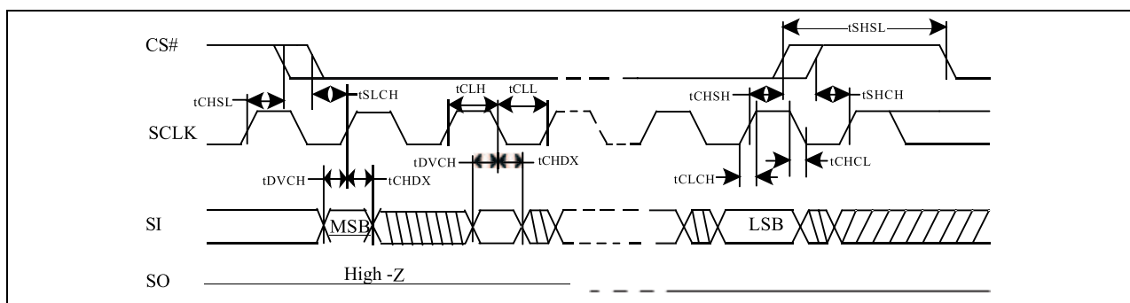
Figure 9-5 Output Timing
