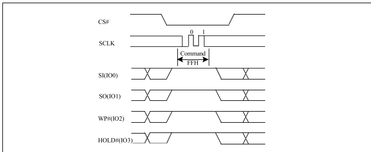
Figure 10-27a Disable QPI Sequence (QPI)
