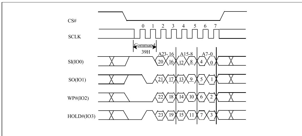
Figure 10-54a Individual Block Unlock (QPI)
