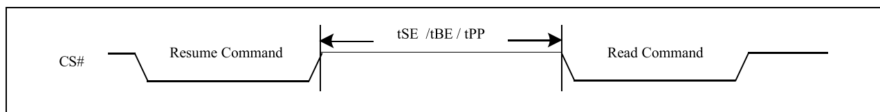
Figure 10-51 Resume to Read Latency
