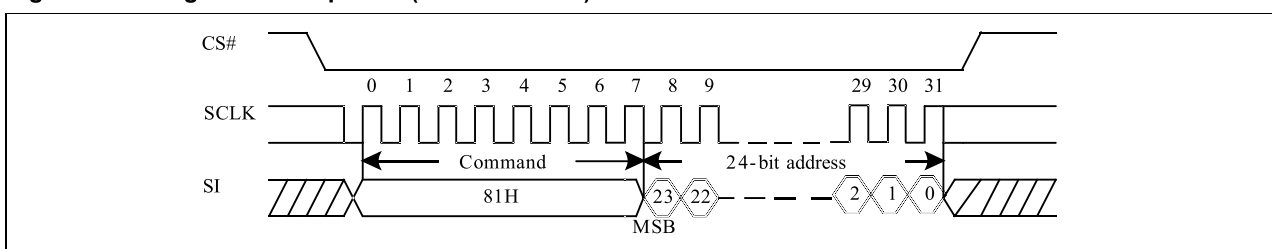
Figure 10-28 Page Erase Sequence (Command 81h)
