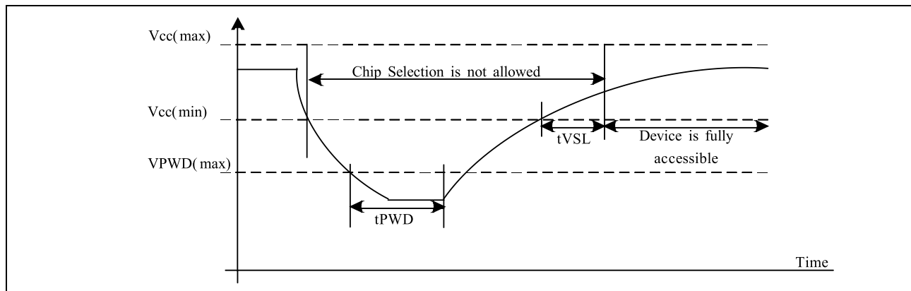
Figure 9-10 Power down-up Timing
