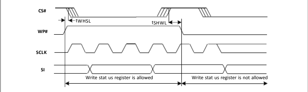
Figure-50. WP Timing
