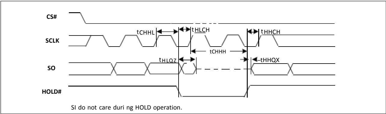
Figure-49. Hold Timing
