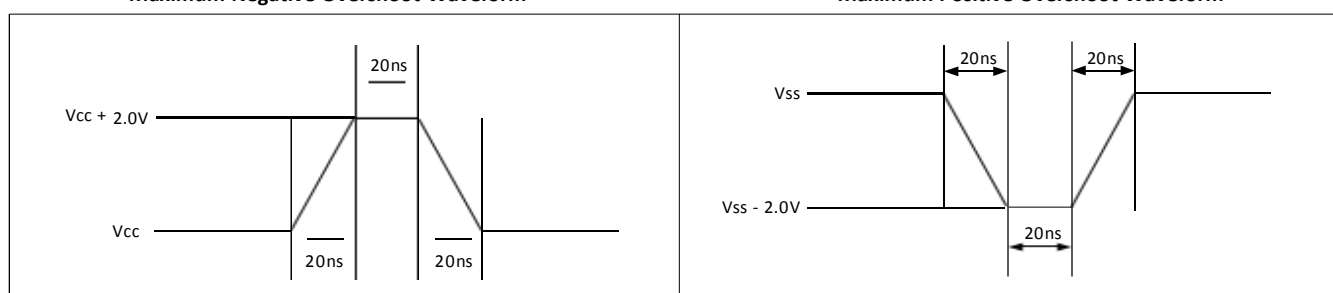
Maximum Positive Overshoot Waveform
