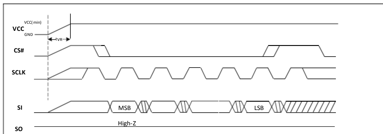
Figure- 4 5. Power- On Timing Sequence Diagram
