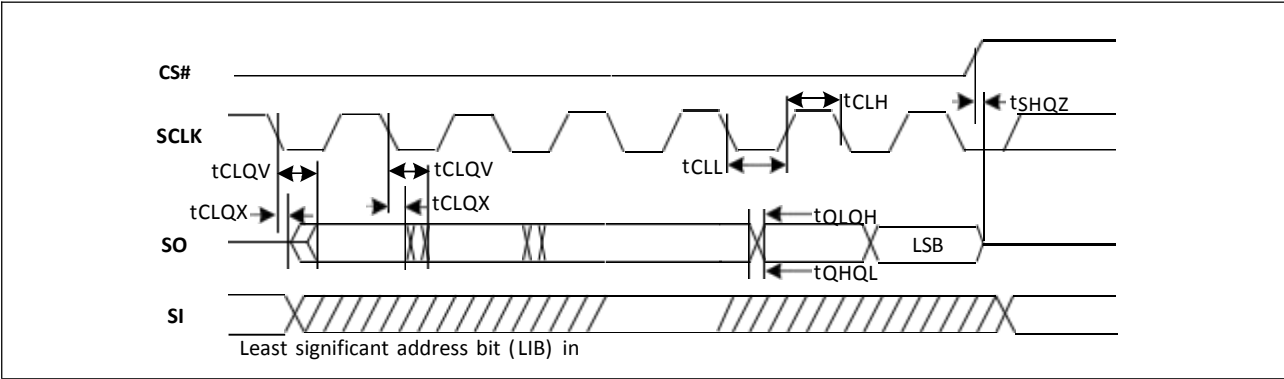
Figure-48. Output Timing
