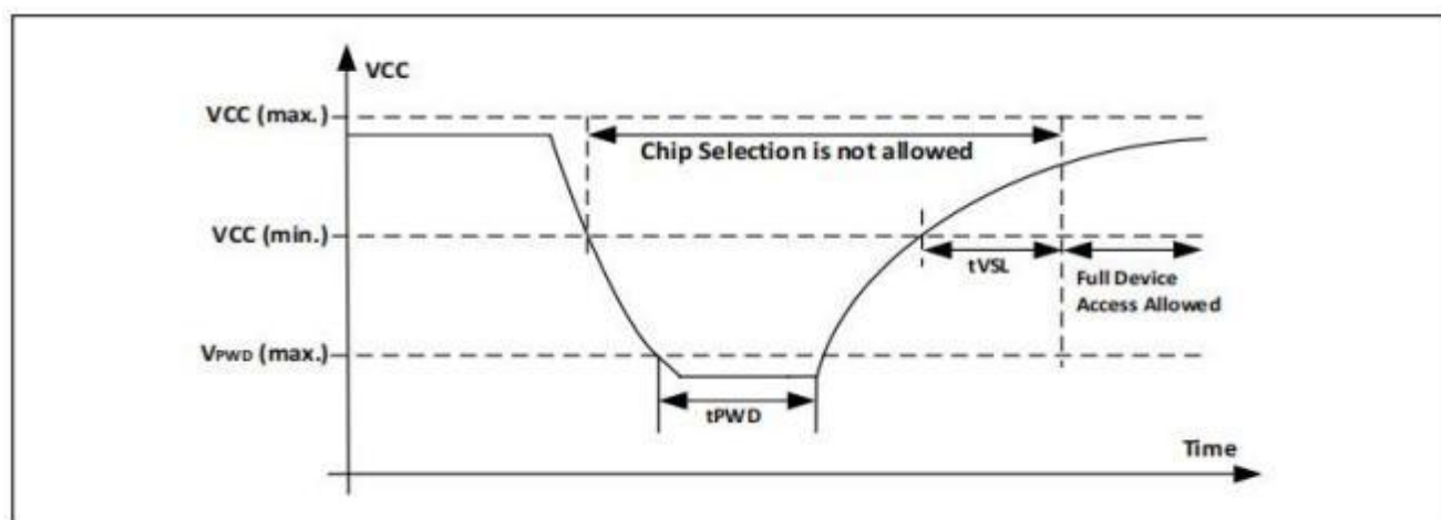
Figure- 4 5. Power- On Timing Sequence Diagram
