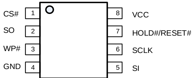
Figure 3-1 for SOP8 and TSSOP8 package
