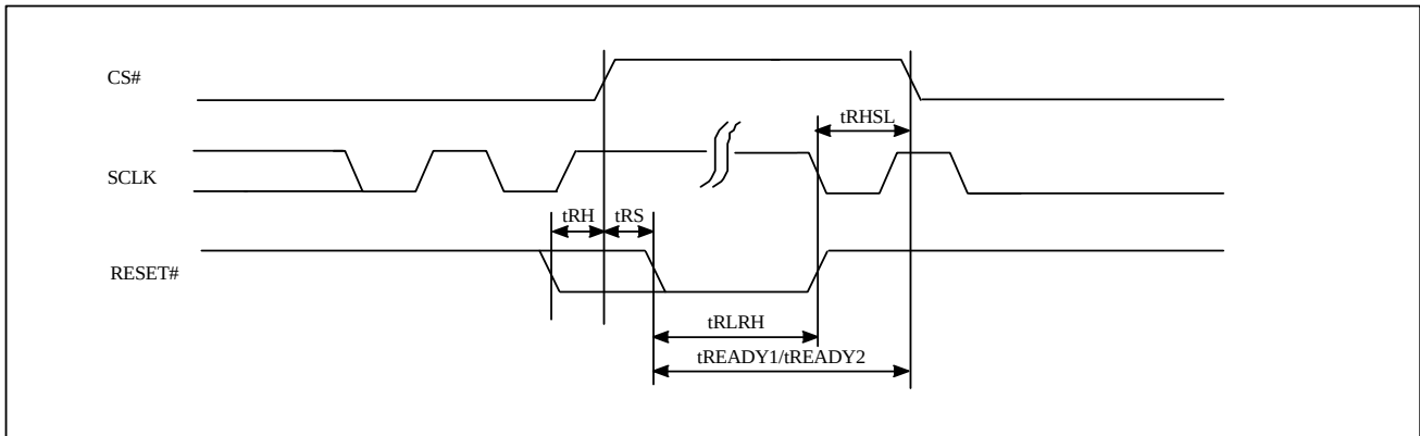
Figure 10-57 Reset Timing
