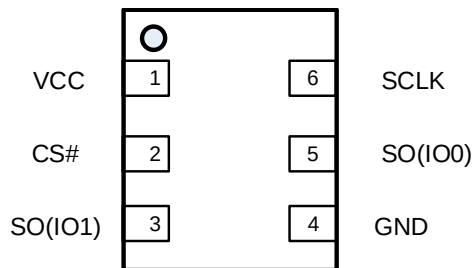
Figure 3-3 for USON6 package
