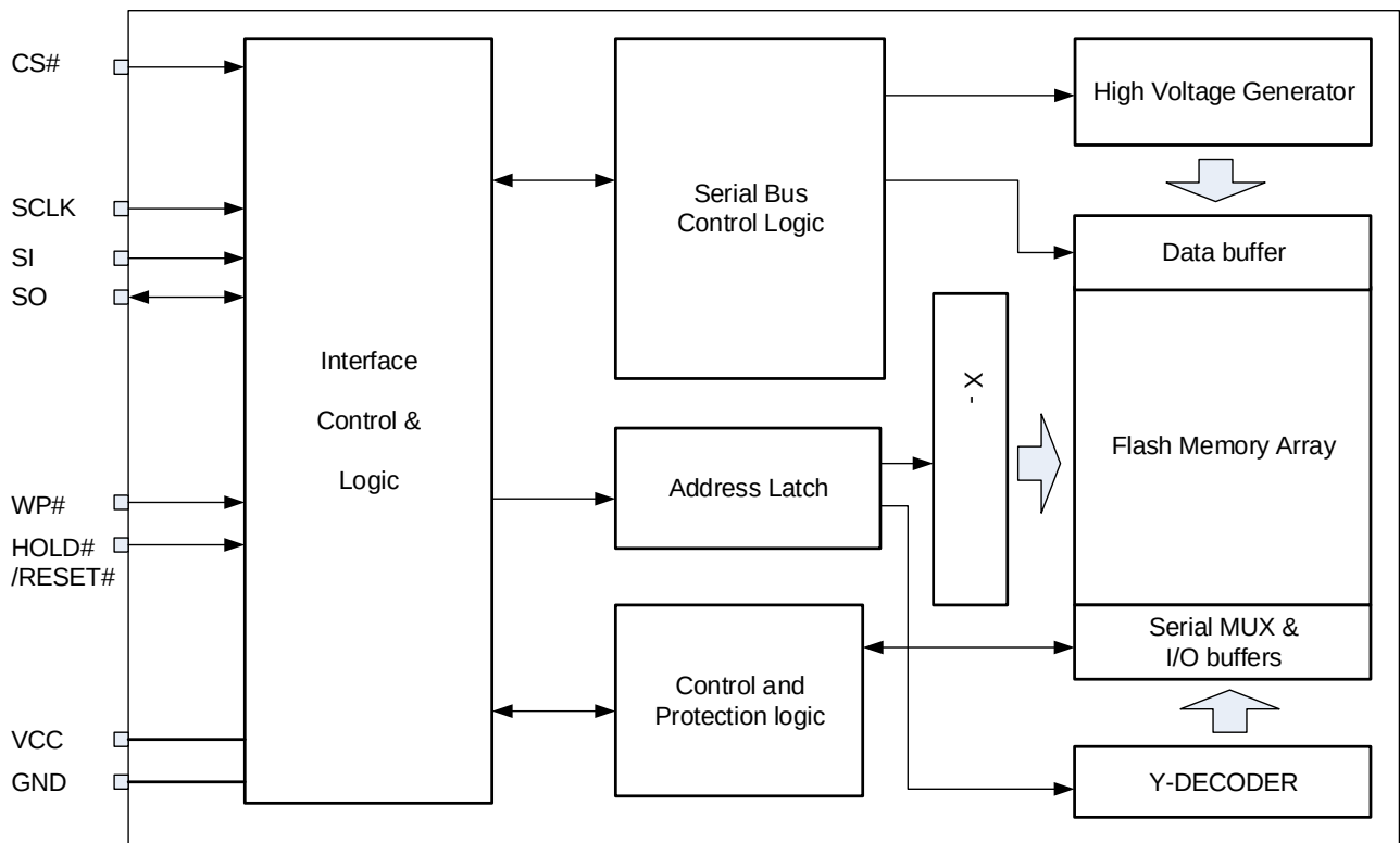
Block Diagram
