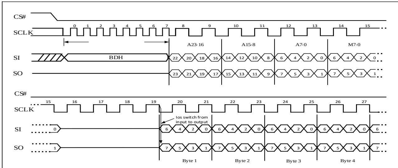
Figure 10-14 DTR 2IO Read Sequence (Command BD M5-4 ≠ (1,0))
