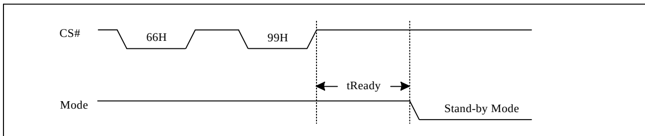
Figure 10-56a Reset Sequence
